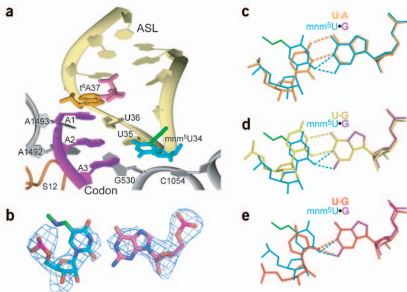
Figure 4 mnm^5U \cdot G , U-A and U•G base pairs. (a) Overview of the decoding site for ASL Lys UUU - mnm^5U34 , t^6A37 -AAG. 16S rRNA is gray, with interacting bases drawn, S12 is orange, codon is purple, and ASL is cream. The base of t^6A37 is orange, and the modification is pink; the base of mnm^5U34 is cyan, and the modification is green. (b) mnm^5U34 \cdot G3 base pair (carbons for mnm^5U34 base are cyan and for modification are green; carbons for G3 are purple) is shown with electron density ( 2F_o - F_c contoured at 1.5 \sigma ). (c) mnm^5U34 \cdot G3 (cyan and green) and U34•A3 (orange) are superimposed by alignment of nonvariant 16S rRNA phosphate atoms, with anticodon at left and codon at right. The U34•A3 base pair represents the classic Watson-Crick geometry. (d) mnm^5U34 \cdot G3 (cyan and green) and G36•U1 from the X-ray structure of the 30S ribosome bound to noncognate tRNAs 3 (yellow) are superimposed by alignment of the G nucleotide. The G36•U1 base pair is a classic G•U wobble 4 , but is flipped to align with the mnm^5U34 \cdot G3 base pair. (e) mnm^5U34 \cdot G3 (cyan and green) and U5•G4 (magenta) from the NMR structure of the self-complementary oligonucleotide r(GGCUGGCC)_2 (ref. 32) are superimposed by alignment of the G nucleotide. Both U•G base pairs use bifurcated hydrogen bonds (dashed lines).
